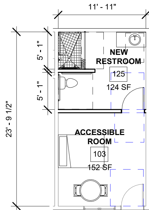
Compliant ADA Unit - 283 sq. ft.
