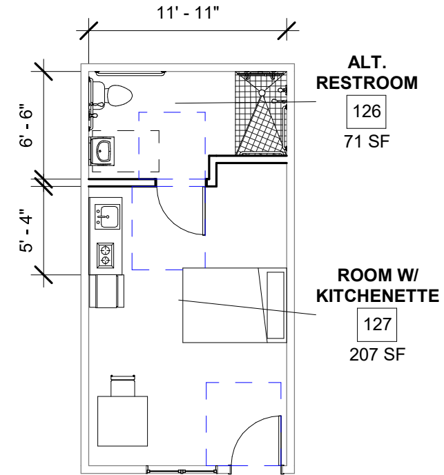
Compliant ADA Unit w/ Kitchen - 283 sq. ft.
